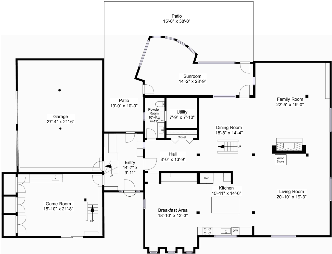
First Floor Plan Ceiling Height = 7'-7"
